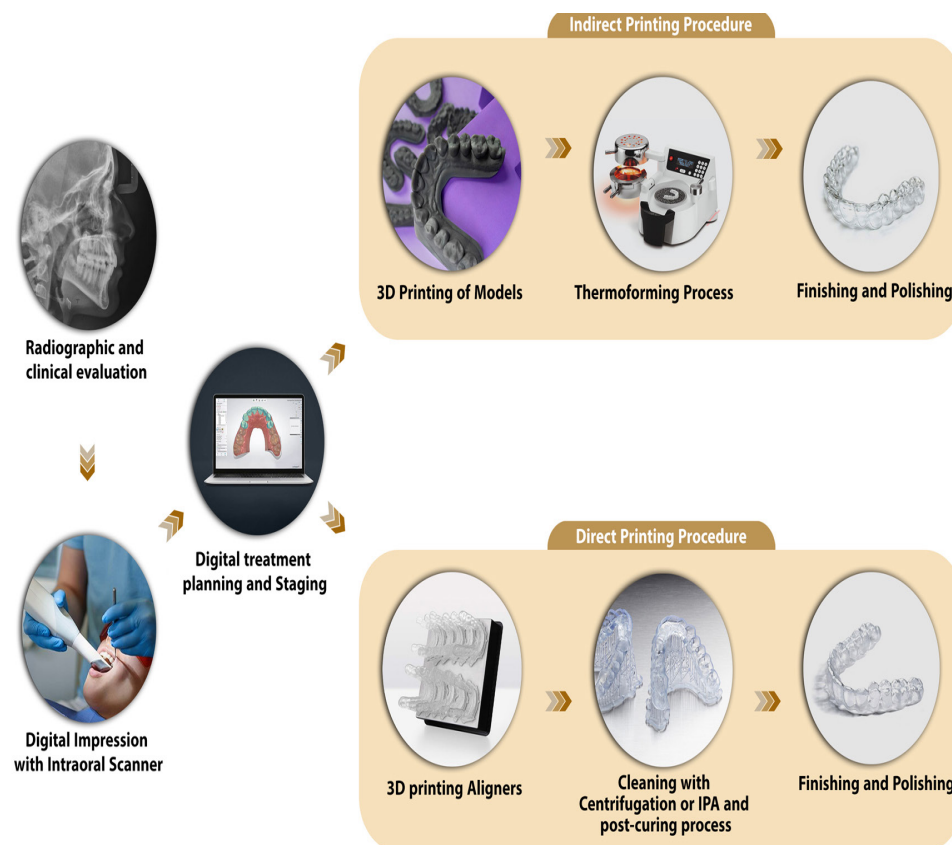
Figure 1. Step-by-Step Workflow of Indirect vs. Direct 3D Printing Process Used in Orthodontic Clear Aligner Fabrication
